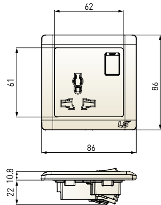
1 gang multi socket with switch
