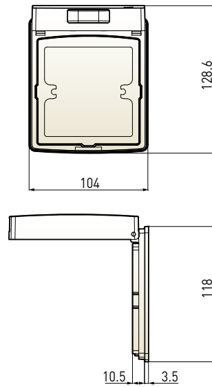
Water proof cover
