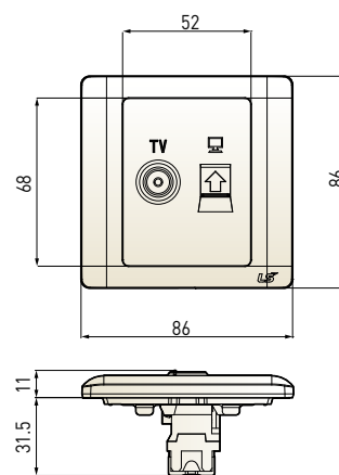
TV+Computer socket
