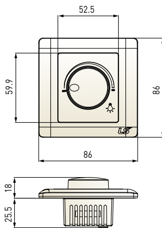
1 gang dimmer switch
