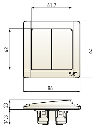
2 gang 2 way switch
