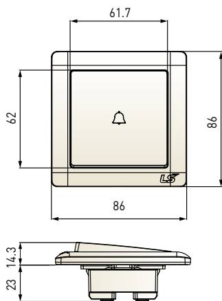
1 gang doorbell switch
