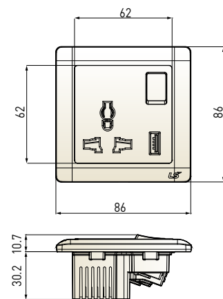
1gang socket with switch+USB
