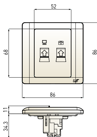
Computer+TEL socket
