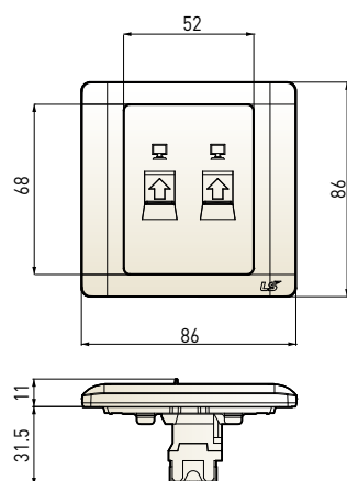
Computer+Computer socket
