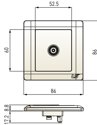
1 Gang TV socket
