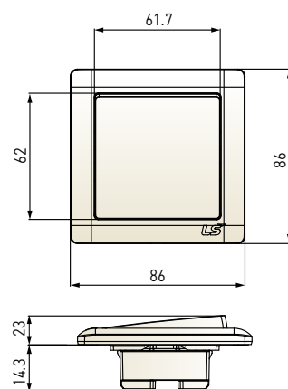
1 gang 2 way switch
