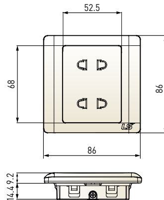
2 Gang 2 pole socket
