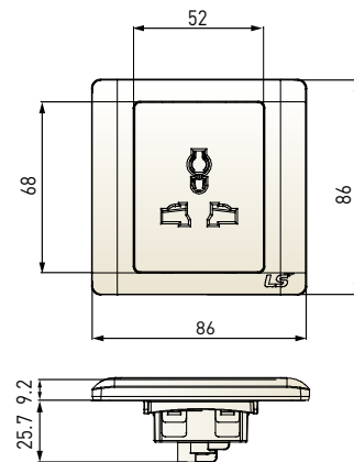
1 gang multi socket
