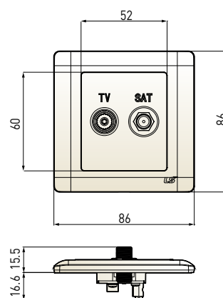
TV+Satellite socket
