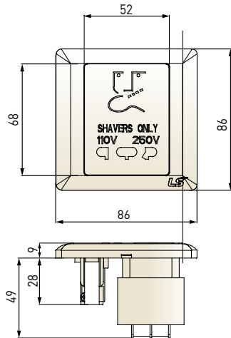
Shaving socket
