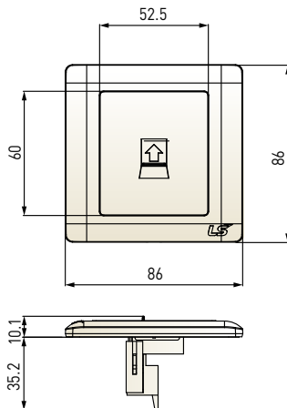
1 Gang computer socket
