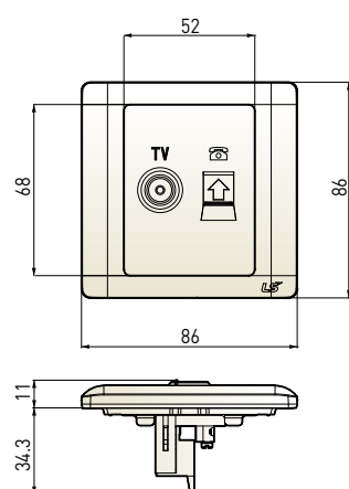
TV+Telephone socket
