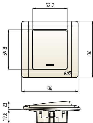
20A heater water switch
