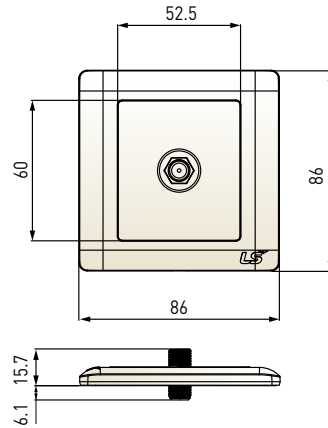
1 gang satellite socket
